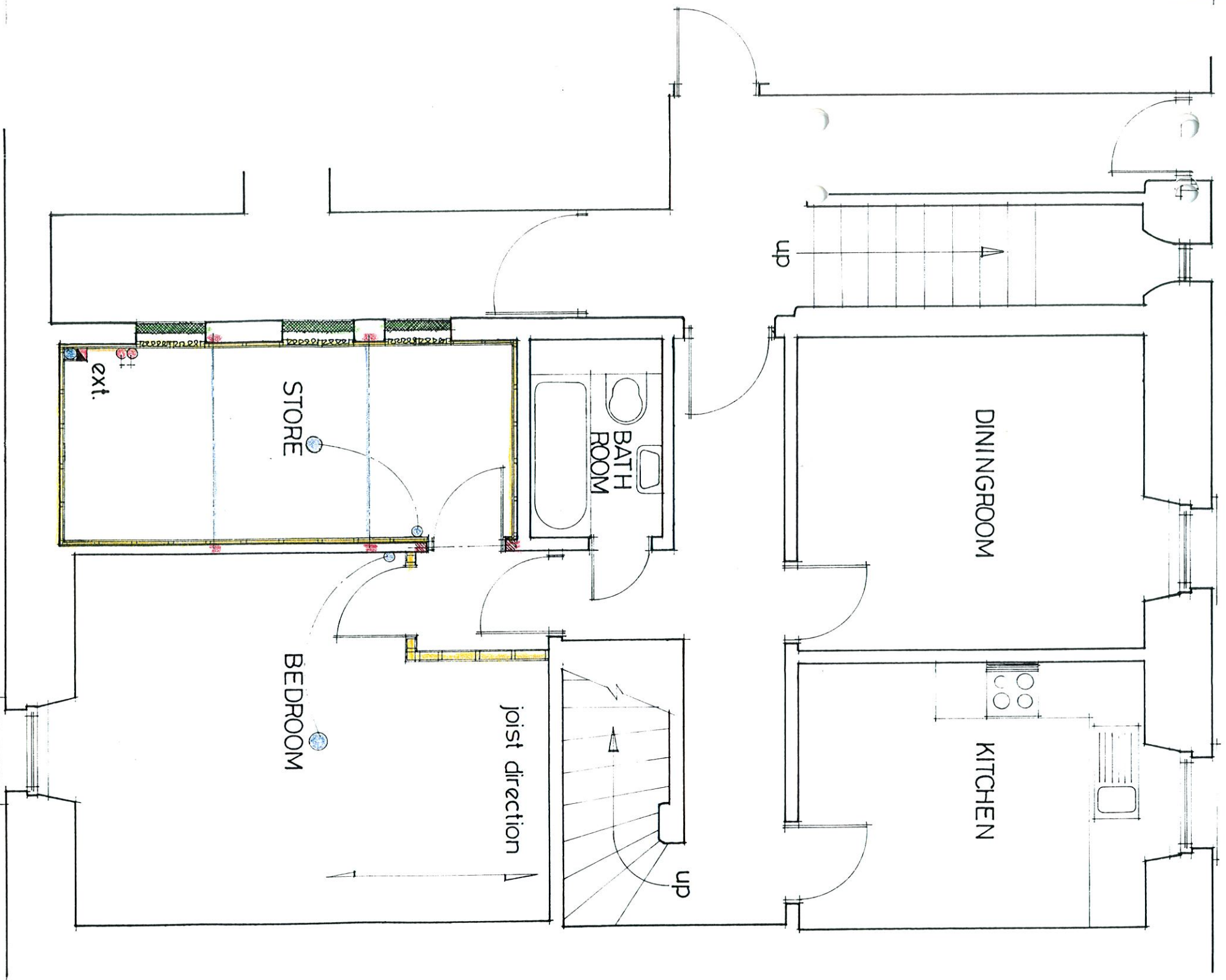
proposed lower ground floor plan
